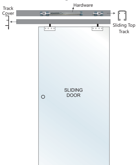
One Way Soft Close Sliding Hardware
