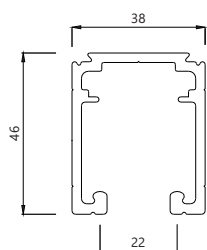
Sliding Top Track CASP-T1
