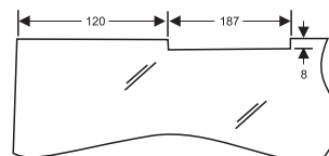
CDC-68 with Saddle Plate (187) with Door Width upto 950mm
