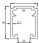
Sliding Top Track CASP-T1-1800/3600mm
