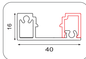
CASP-SHP-4016 (Clip M/F Set)
