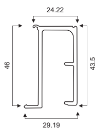
Track for Fix Glass CASP-FG-T1
