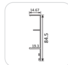
Track Cover : CASP-TC-T1
