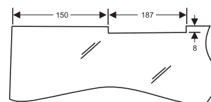
CDC-68 with Saddle Plate (187) with Door Width upto 1100mm
