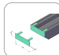
CAP-4011 Aluminium Casted ₹ : 250.00 (in all 5 Finish)
