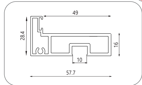
Slim Outer Frame Profile CASP-OFP-1351
