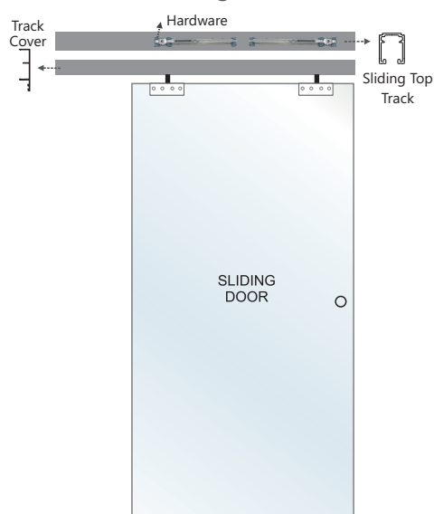
Two Way Soft Close Sliding Hardware
