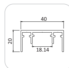
Bottom Profile CASP-4013
