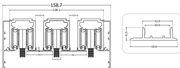
TopTrack Concealer with Clip on : CASP-1411 (Optional)
